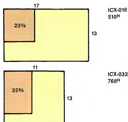
Figure 4. The smaller pixel size in the HAD sensor is more than offset by the larger opening ratio, which effectively increases the sensor's sensitivity.
