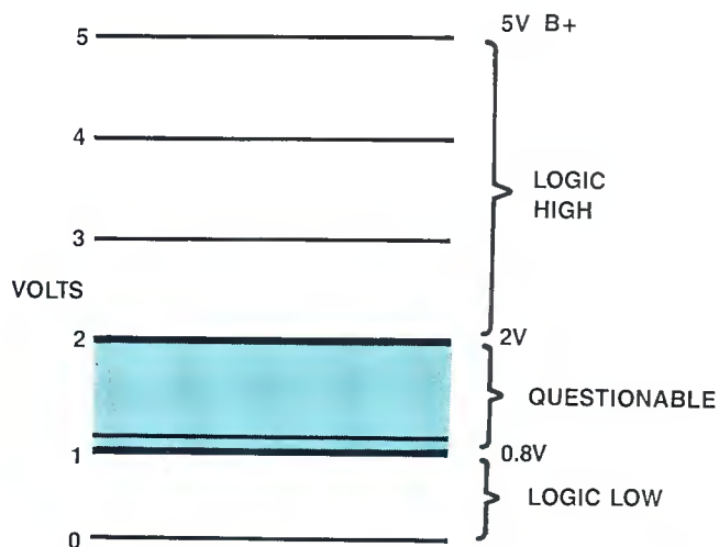
Figure 2. Logic level tolerance envelope for TTL-based systems. (From: Carey, Gregory D. "Isolating Microprocessor-Related Problems." Electronic Servicing and Technology magazine, Intertec Publishing, Overland Park, KS, June 1988.)
