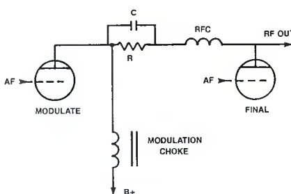
Figure 1. Typical Heising circuit.
