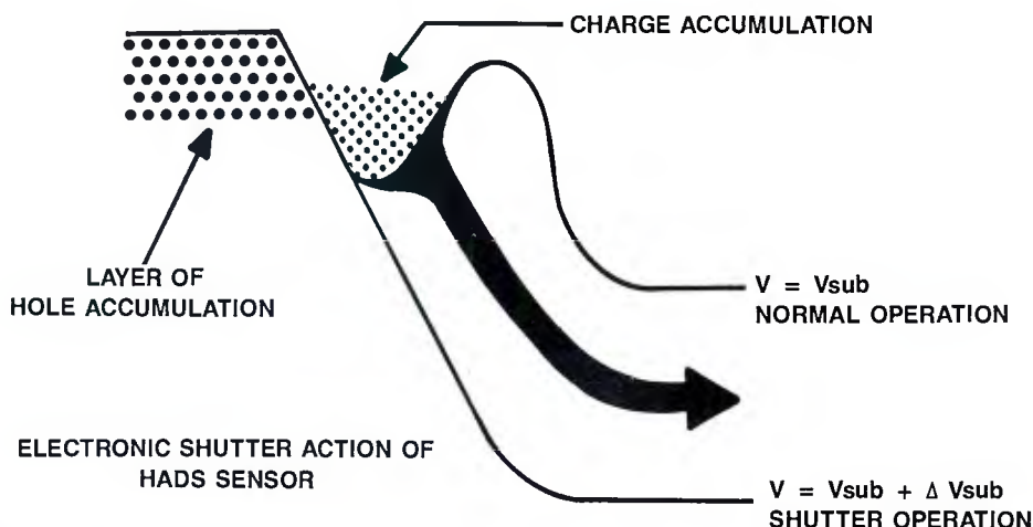
Figure 6. In a HAD sensor, each pixel has its own electronic shutter. When the shutter is actuated, the substrate is pulsed, lowering the potential barrier of the well and effectively dumping the collected charge.
