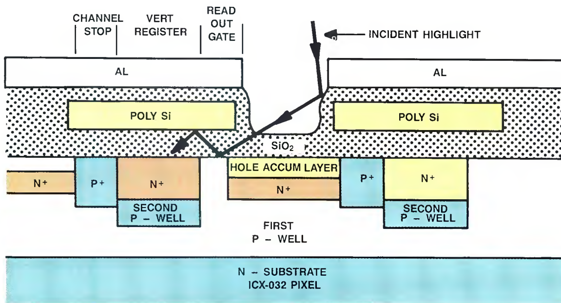
Figure 8. Optical "sneak paths" cause smear when bright highlights are propagated within the CCD and contaminate wells in the registers. Only the most intense of highlights will activate the generation of stray carriers by this means.
