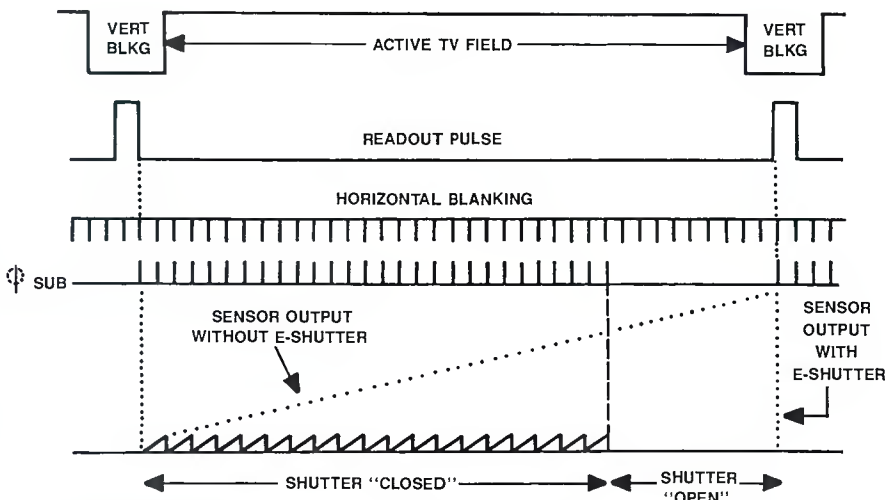
Figure 7. Pulses in the substrate periodically dump the well in a HAD device. This is equivalent to closing a shutter over the device face.
