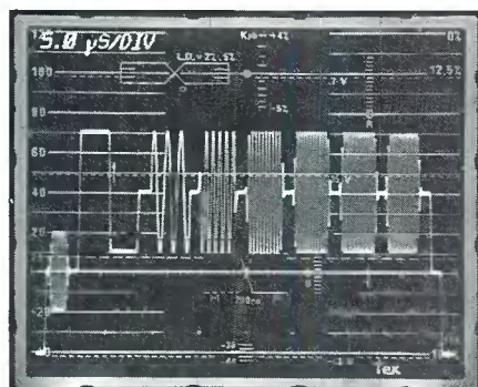
Figure 1a. Multiburst test signal with 0.5MHz, 1MHz, 2MHz, 3MHz, 3.58MHz and 4.2MHz packet frequencies.
