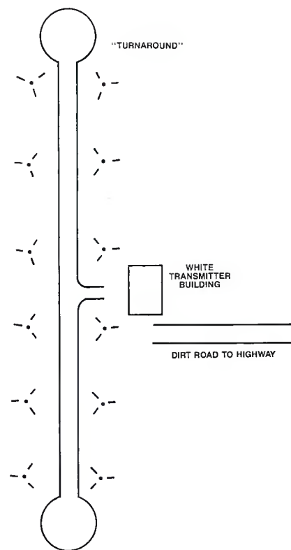
Figure 1. The KLIF array as it appeared in the summer of 1969.
