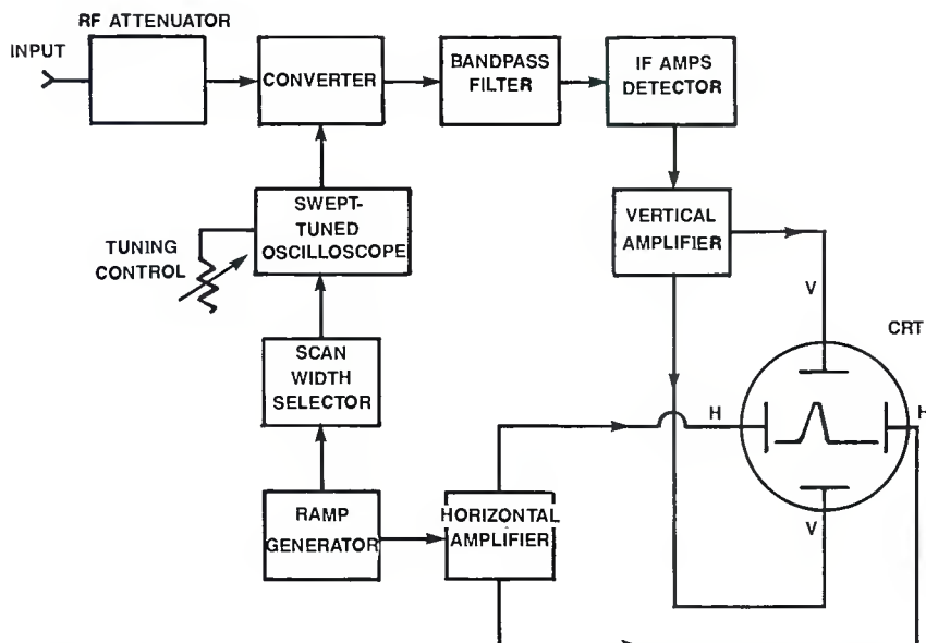
Figure 1. Block diagram of a spectrum analyzer. (From Kinley, Harold. "Using Service Monitor/Spectrum Analyzer Combos." Mobile Radio Technology magazine, Intertec Publishing, Overland Park, KS, July 1987.)
